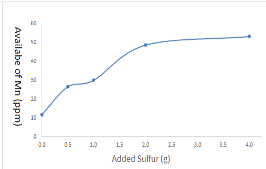
Figure 1: Effect of Sulfur addition to soil on Mn release.
